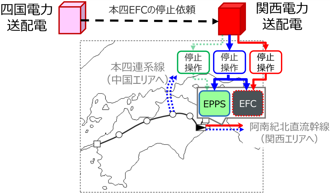
[直流潮流]
